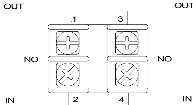
Figure 2: Terminal Block
