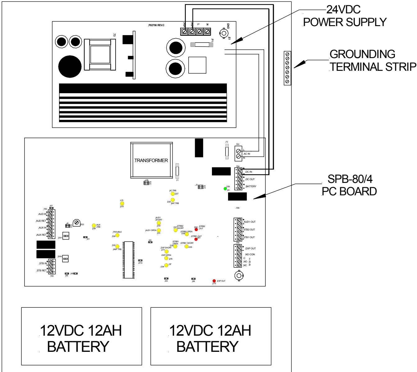
Figure 2-3 Layout of SPB-80/4 SAFEPATH4 Audio Booster Panel
