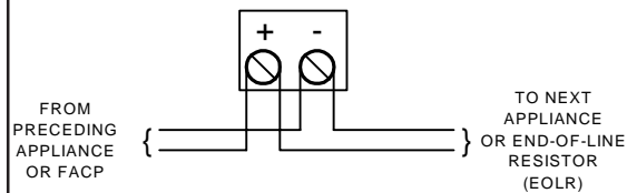
Fig. 1 Bell Models
